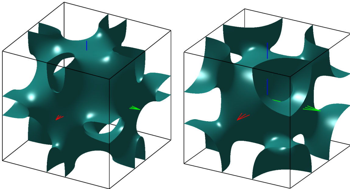
Figure 1: Left: Nodal approximation of the Neovius surface. Right: Nodal approximation of the Schwarz I-WP surface. The ranges are -\pi \leq x, y, z \leq \pi in both plots, the red, green and blue arrows are the vectors (\pi, 0, 0) , (0, \pi, 0) and (0, 0, \pi) , respectively.
